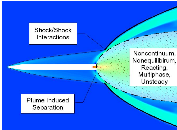
High Altitude Missile/Rocket Plumes CONVENTIONAL PROBLEM
